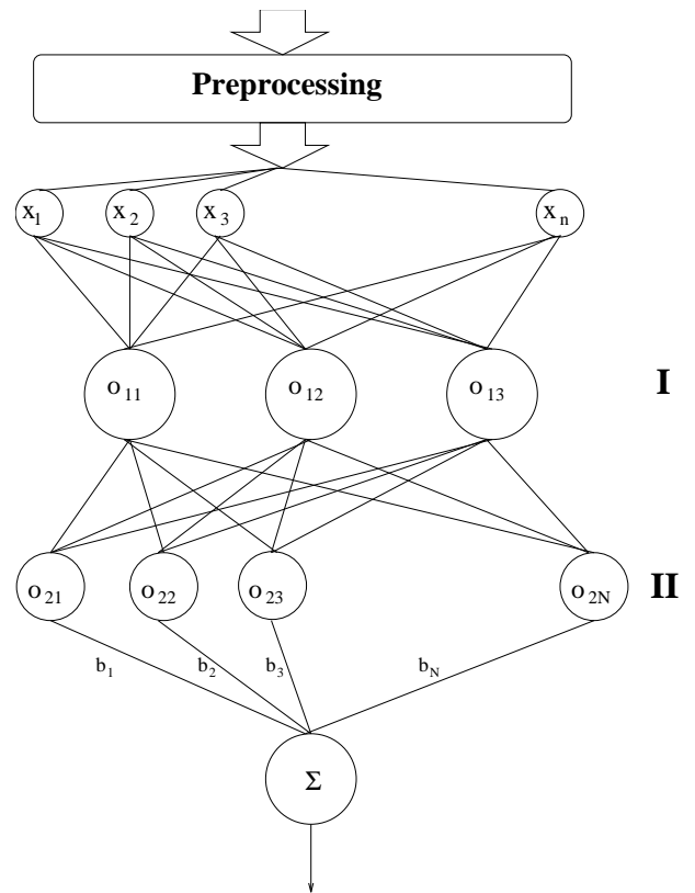
Fig. 19. An approximation network for template matching. The preprocessing stage applies simple transformation to the input pattern (e.g. to emphasize high frequency components).
