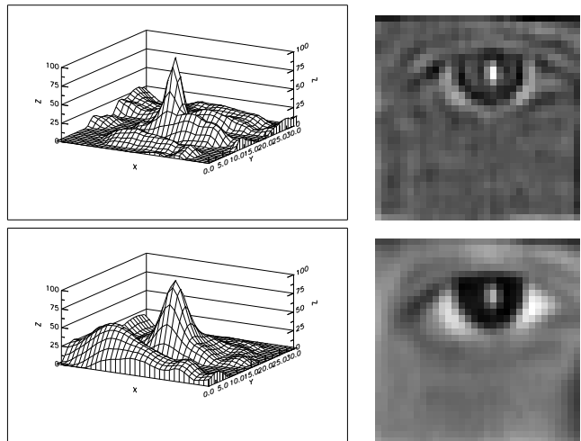
Fig. 5. Using an increasing amount of added white noise the emphasis given to the high frequency is reduced and the resulting filter response approaches that of the standard MSF.
