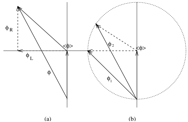
Fig. 9. Computing the distance from linear subspace (a) versus computing the distance from a single prototype (b). In drawing (a), vector \langle \phi \rangle represents the average pattern and the horizontal line on which \phi_L lies represents the linear subspace. \phi_L is the projection of pattern \phi on the linear space and \phi_R is the projection residual. Drawing (b) shows two vectors \vec{\phi}_1 and \vec{\phi}_2 with the same distance from the average pattern \mathbf{A} but different distances from the pattern space.
