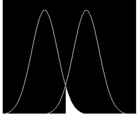
Fig. 1. The probability of error, represented by the shaded area, when the distributions are Gaussian with the same covariance.
