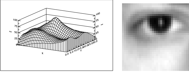
Fig. 2. The cross-correlation of the template reported on the right. Note the diffuse shape of the peak that makes its localization difficult
