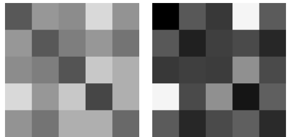
Fig. 10. The square of coordinates ij represents the average value of distances of views of the i -th and j -th clip (darker values represent smaller distances). LEFT: euclidean distances of views of the different clips; RIGHT: distances computed using the learned metric W_0^T W_0
