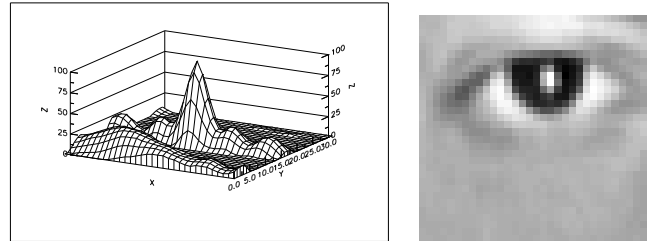
Fig. 8. Non linear processing can be employed. The figure represent the result of preprocessing the image to extract the local image contrast (intensity value over the average value in a small neighborhood). This kind of preprocessing emphasizes high frequencies and results in a sharp correlation peak.
