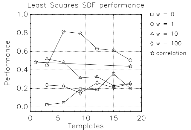
Fig. 18. Performance of least squares SDF with different amount of regularizing noise. Correlation performance is also reported using the average template and the whole set of available templates. The horizontal axis reports the number of patterns used in building the filters, while the vertical axis reports the percentage of eyes correctly located (see text for a detailed explanation).
