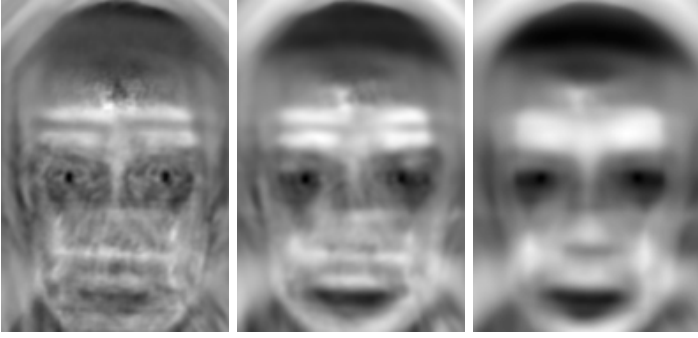
Fig. 6. The output of the correlation with an SDF computed using the spectral envelope of 10 training images and different amounts of white noise (left: \alpha = 1 , middle \alpha = 5 ) compared to the output of normalized cross-correlation using one of the images used to build the SDF but without any spectral enhancement. The darker the image the higher the corresponding value. Note that an increased amount of white noise improves the response of the filter.
