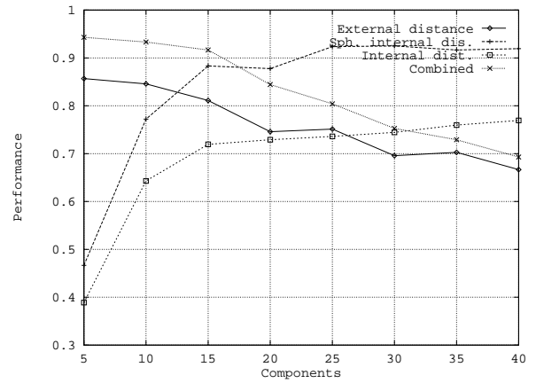
Fig. 17. Performance of different strategies based on the computation of principal components. The horizontal axis reports the number of principal components used in the expansion, while the vertical axis reports the percentage of eyes correctly located (see text for a detailed explanation).
