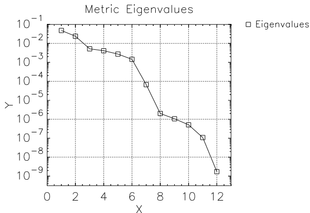
Fig. 11. Eigenvalues of the learned metric matrix \mathbf{W}^T \mathbf{W} . Note that there is compatibility with the findings of Basri-Ullman that under orthographic projection the rank of the metric is 6.
