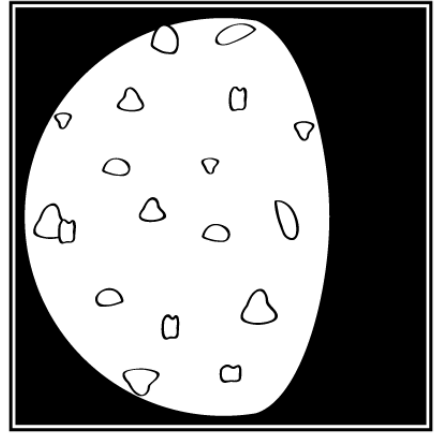
Waning Gibbous
