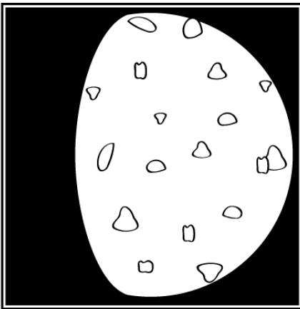
Waxing Gibbous
