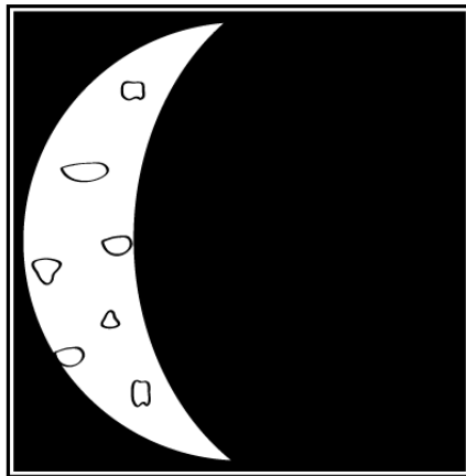
Waning Crescent
