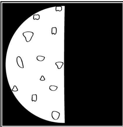
Last Quarter
