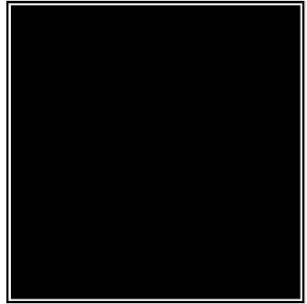
New Moon
