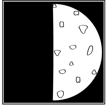
First Quarter
