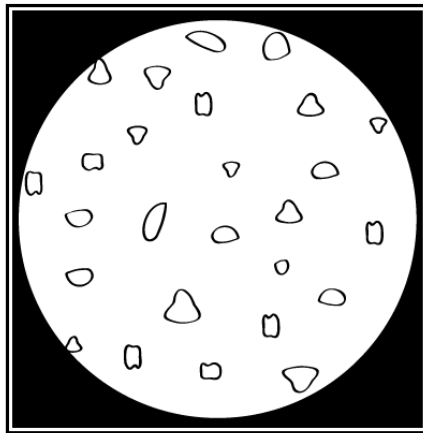
Full Moon
