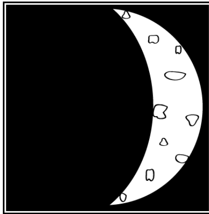
Waxing Crescent
